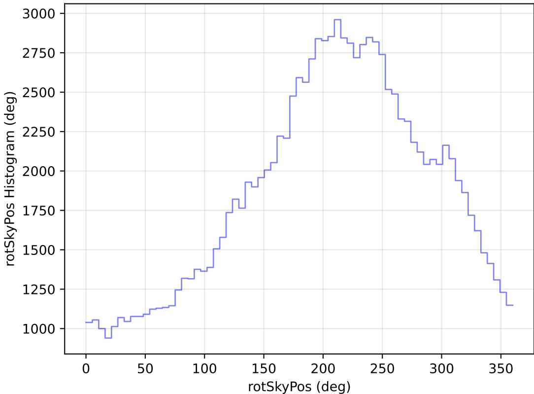
weather_cloudso1v3.4_10yrs All sky u band: rotSkyPos Histogram
