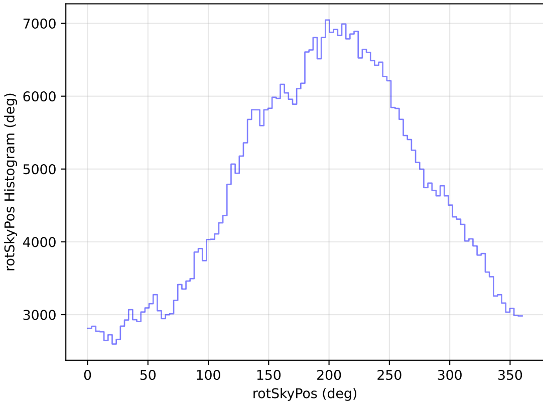
weather_cloudso1v3.4_10yrs All sky r band: rotSkyPos Histogram
