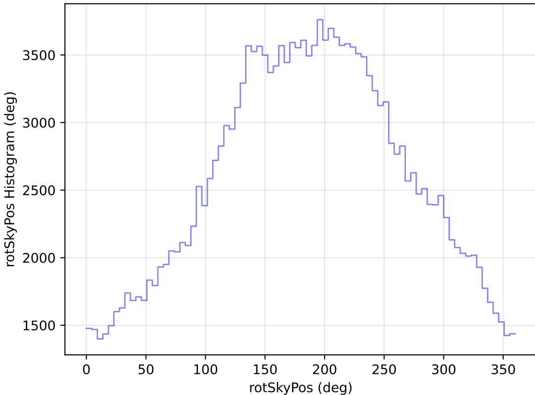
weather_cloudso1v3.4_10yrs All sky g band: rotSkyPos Histogram
