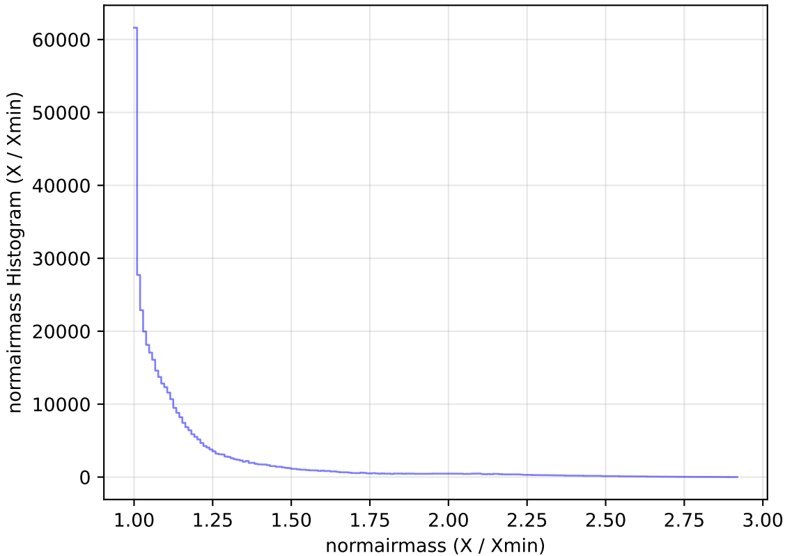
weather_cloudso1v3.4_10yrs WFD z band: normairmass Histogram
