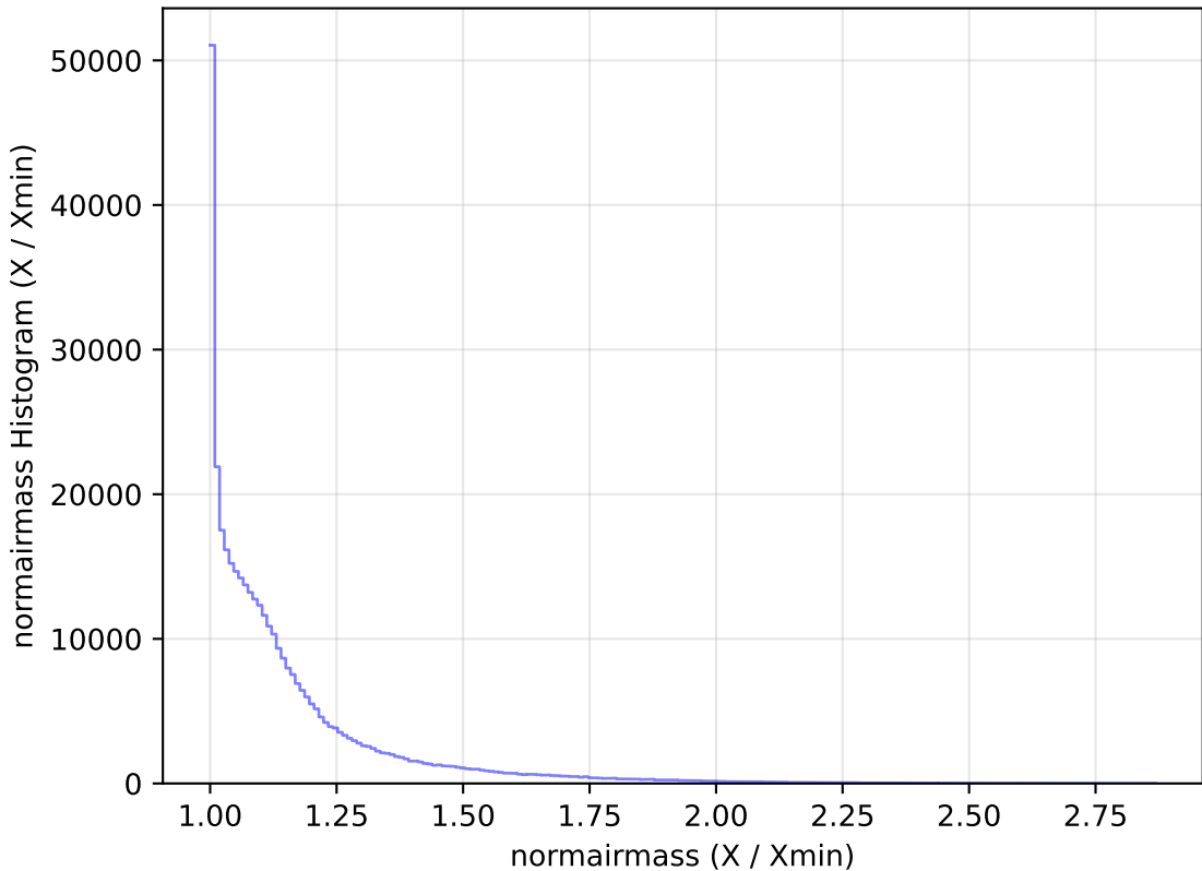
weather_cloudso1v3.4_10yrs WFD y band: normairmass Histogram
