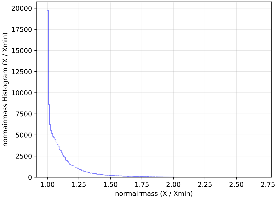
weather_cloudso1v3.4_10yrs WFD u band: normairmass Histogram
