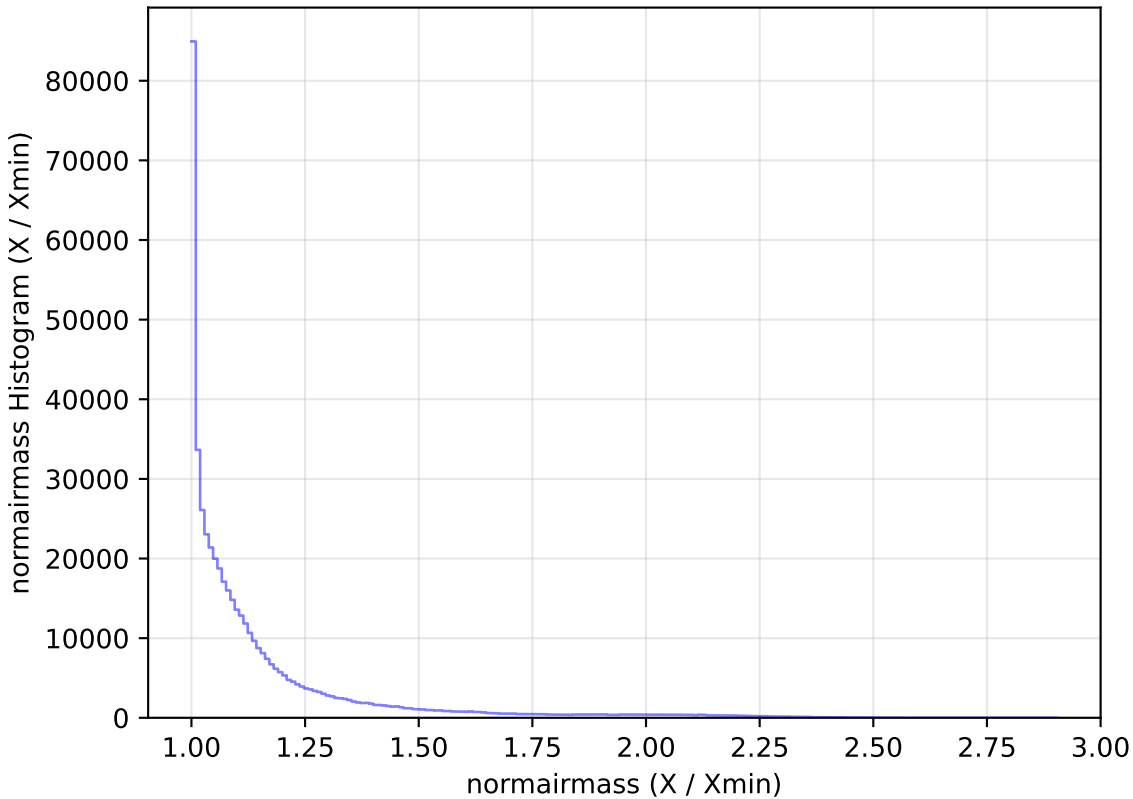
weather_cloudso1v3.4_10yrs WFD r band: normairmass Histogram
