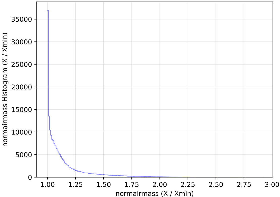
weather_cloudso1v3.4_10yrs WFD g band: normairmass Histogram
