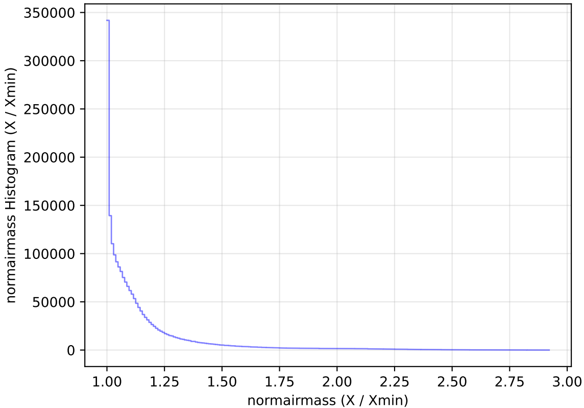
weather_cloudso1v3.4_10yrs WFD all bands: normairmass Histogram
