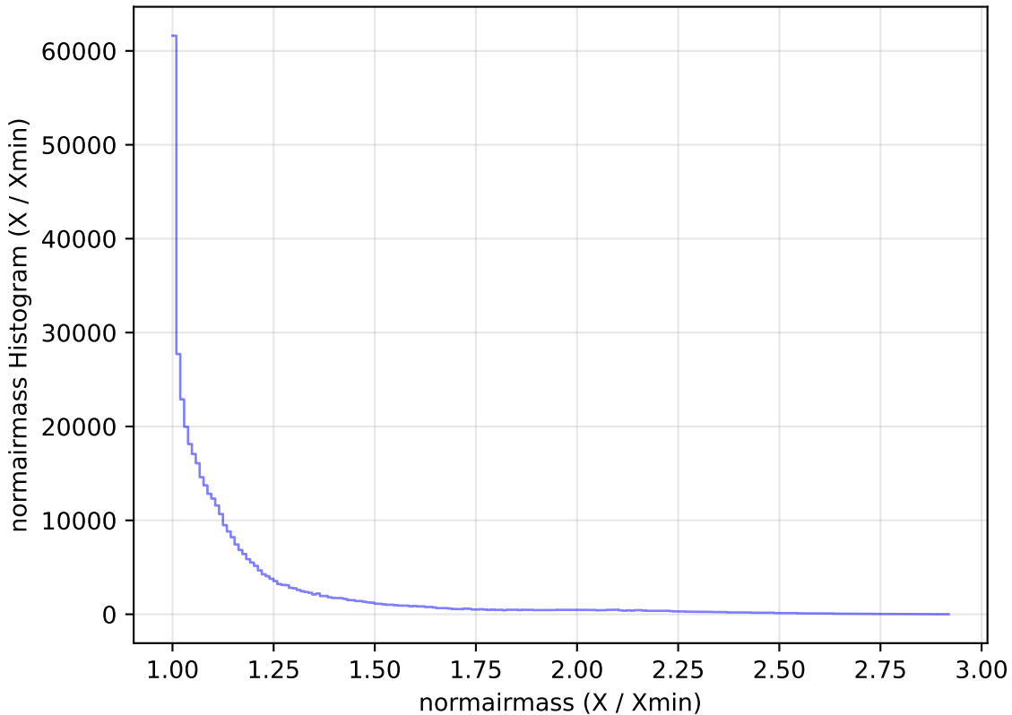
weather_cloudso1v3.4_10yrs All sky z band: normairmass Histogram
