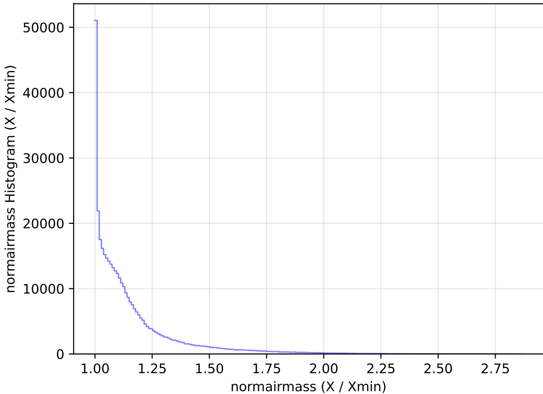
weather_cloudso1v3.4_10yrs All sky y band: normairmass Histogram
