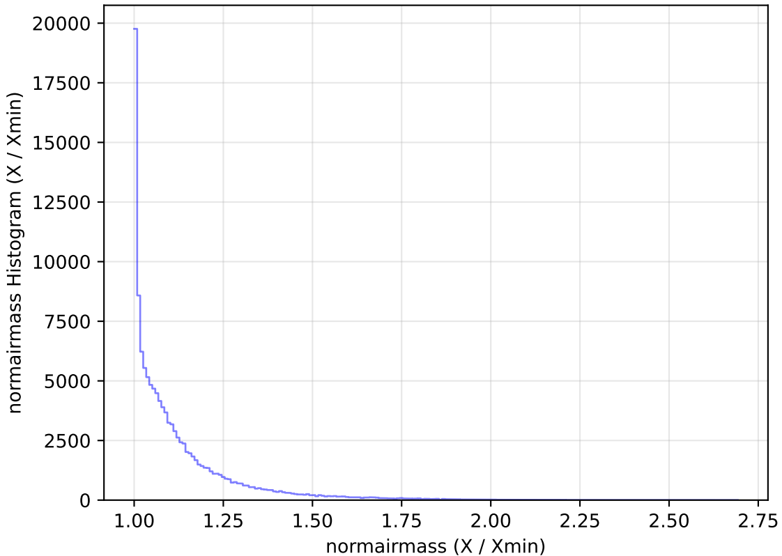
weather_cloudso1v3.4_10yrs All sky u band: normairmass Histogram
