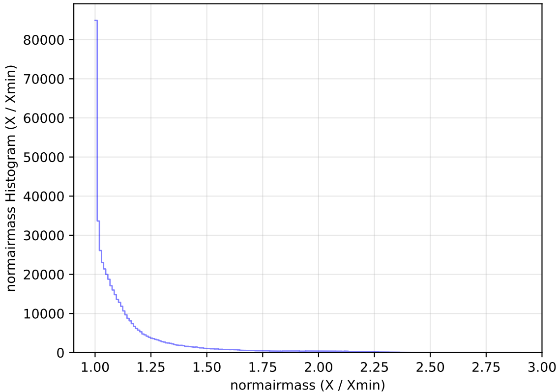
weather_cloudso1v3.4_10yrs All sky r band: normairmass Histogram
