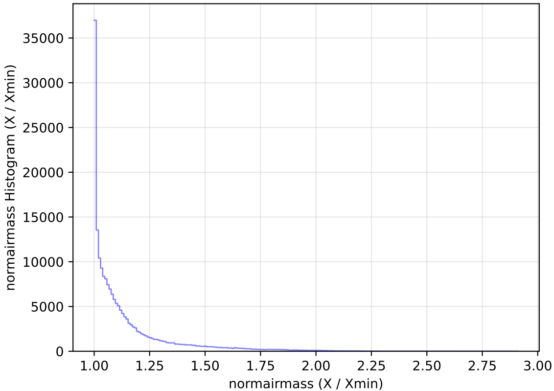
weather_cloudso1v3.4_10yrs All sky g band: normairmass Histogram
