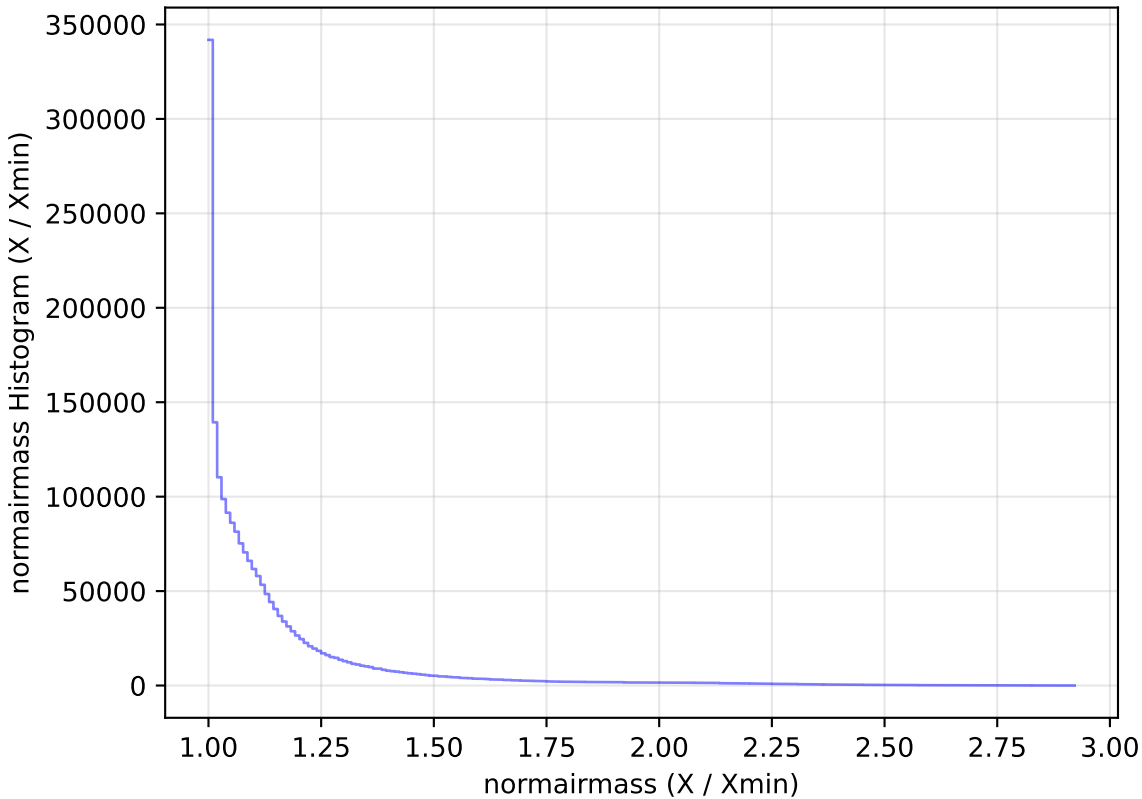
weather_cloudso1v3.4_10yrs All sky all bands: normairmass Histogram
