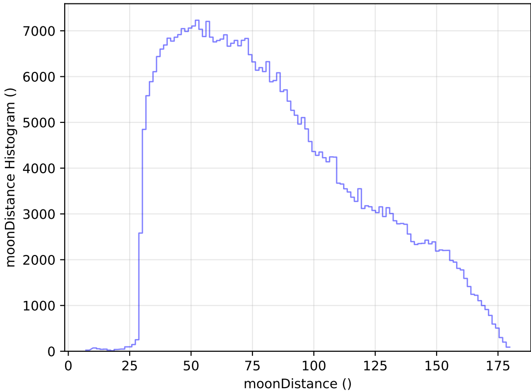
weather_cloudso1v3.4_10yrs WFD z band: moonDistance Histogram
