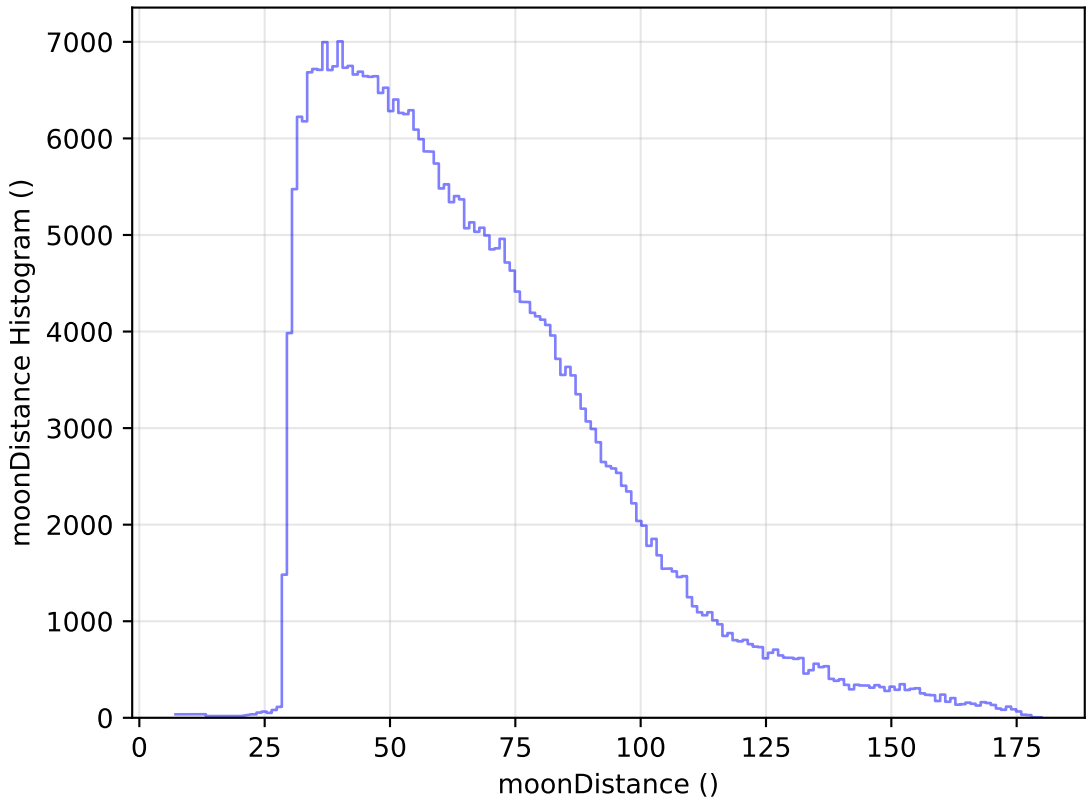
weather_cloudso1v3.4_10yrs WFD y band: moonDistance Histogram
