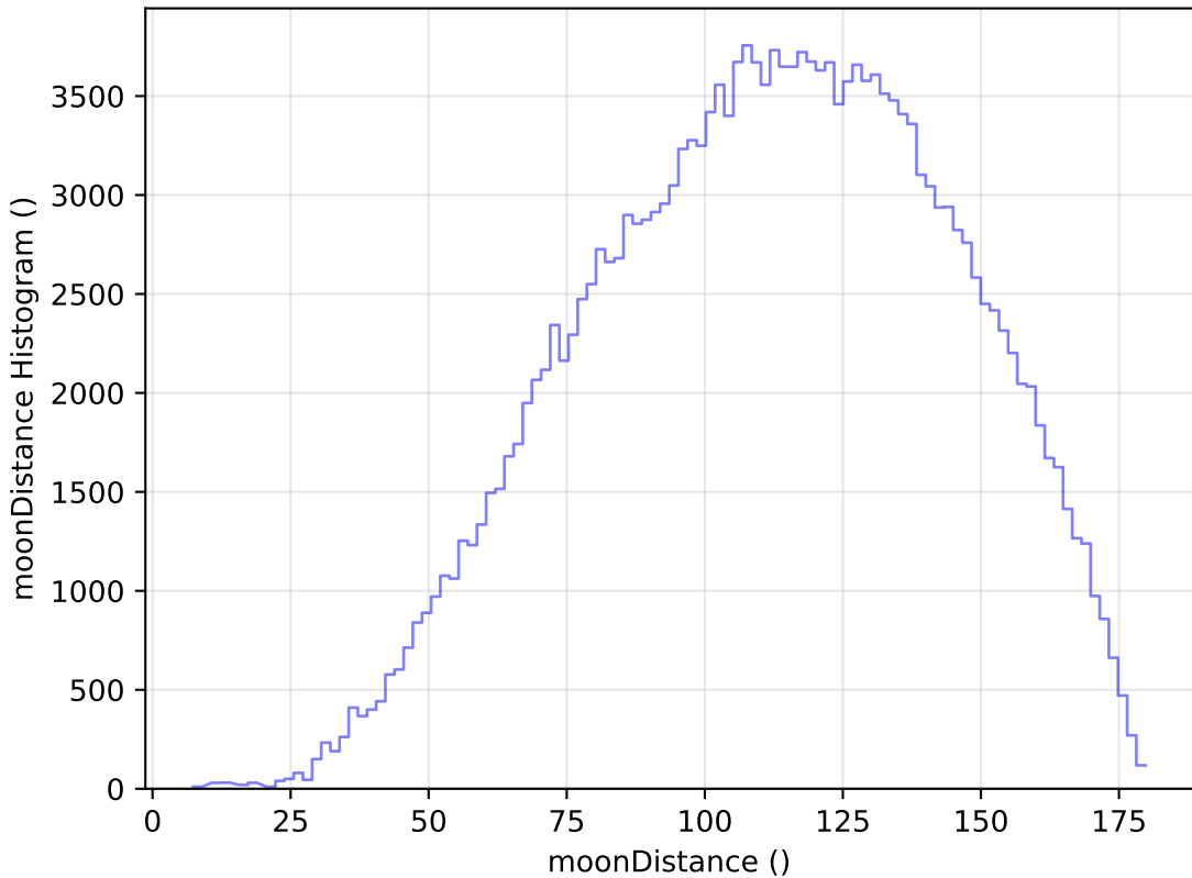
weather_cloudso1v3.4_10yrs WFD g band: moonDistance Histogram
