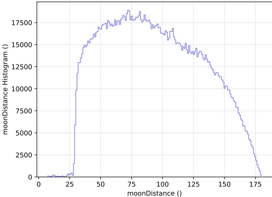
weather_cloudso1v3.4_10yrs WFD all bands: moonDistance Histogram
