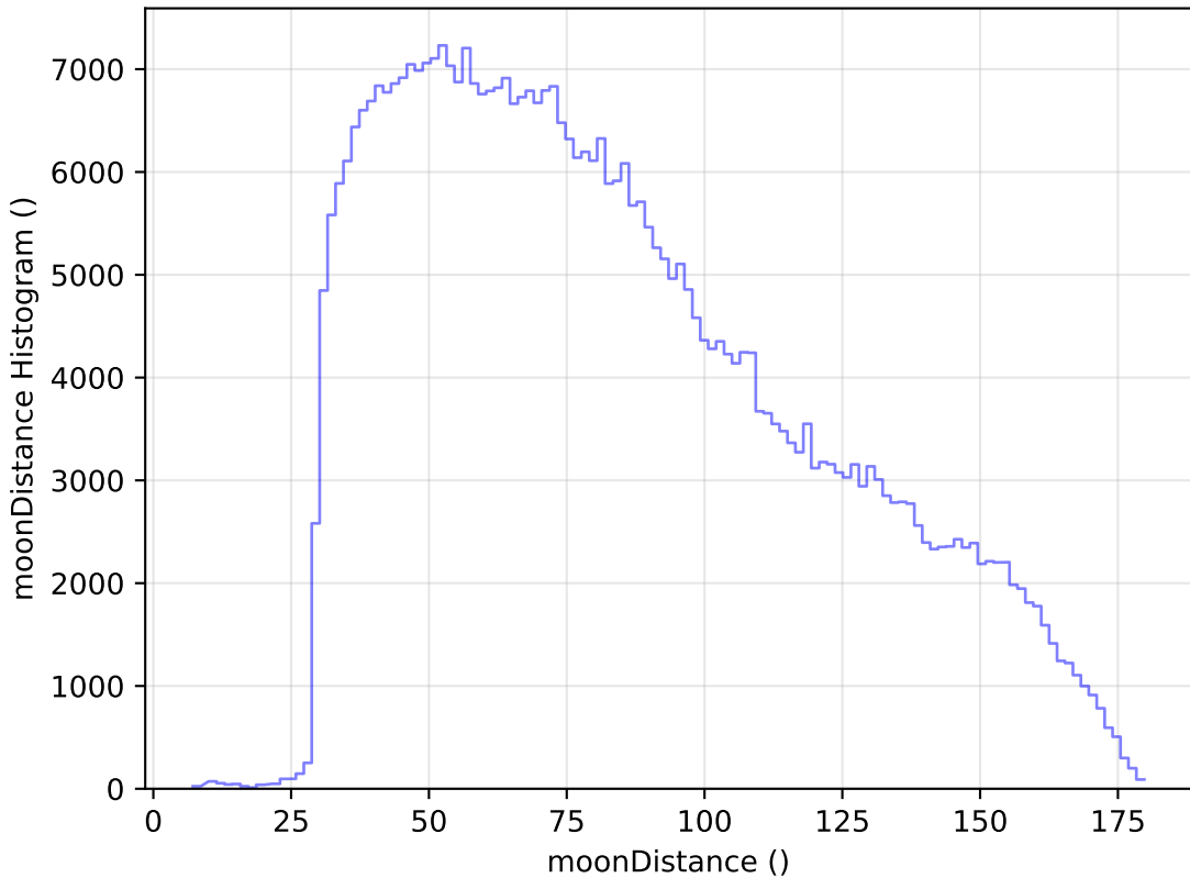
weather_cloudso1v3.4_10yrs All sky z band: moonDistance Histogram
