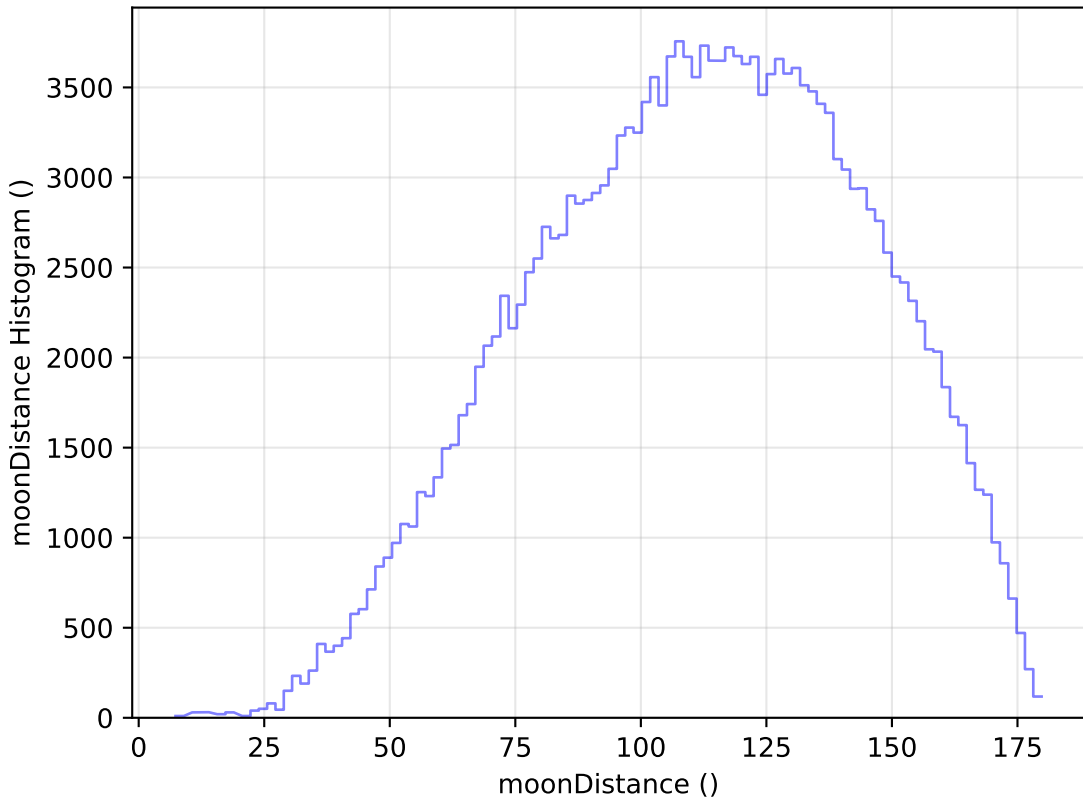
weather_cloudso1v3.4_10yrs All sky g band: moonDistance Histogram
