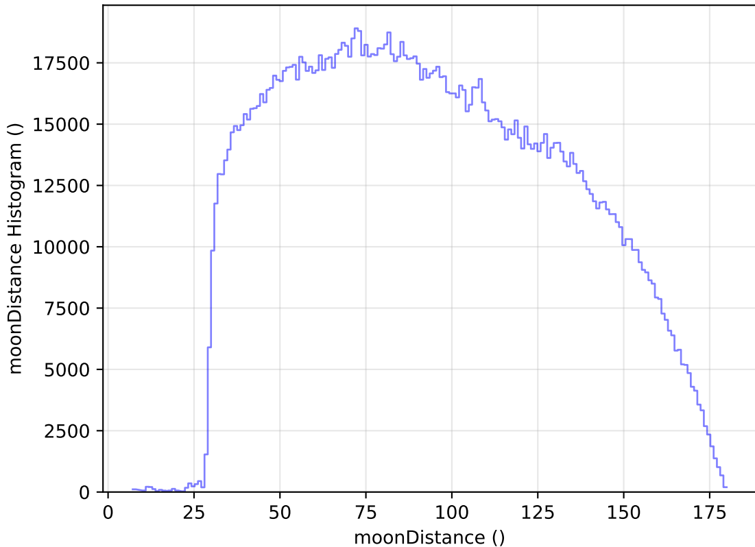
weather_cloudso1v3.4_10yrs All sky all bands: moonDistance Histogram
