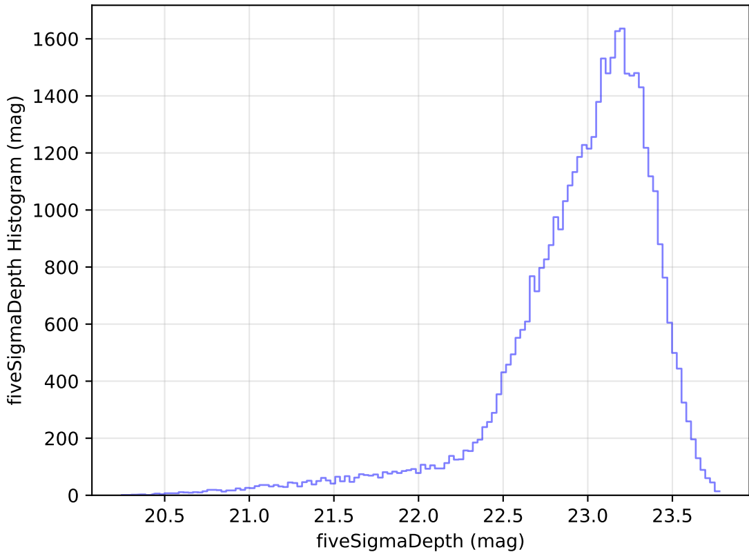
weather_cloudso1v3.4_10yrs Yr 1 z band: fiveSigmaDepth Histogram
