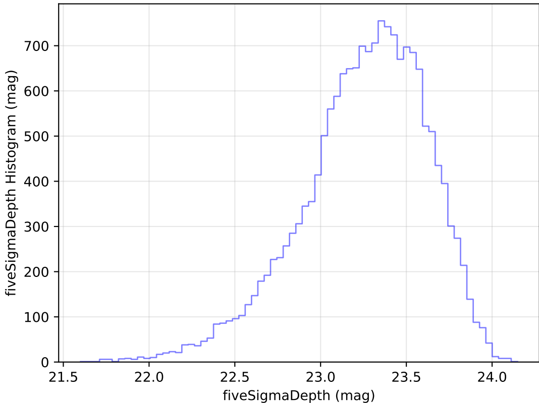
weather_cloudso1v3.4_10yrs Yr 1 u band: fiveSigmaDepth Histogram
