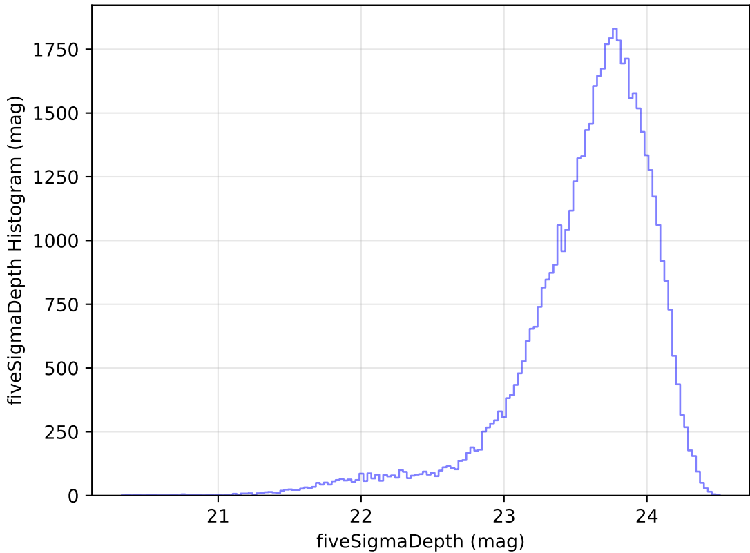
weather_cloudso1v3.4_10yrs Yr 1 i band: fiveSigmaDepth Histogram
