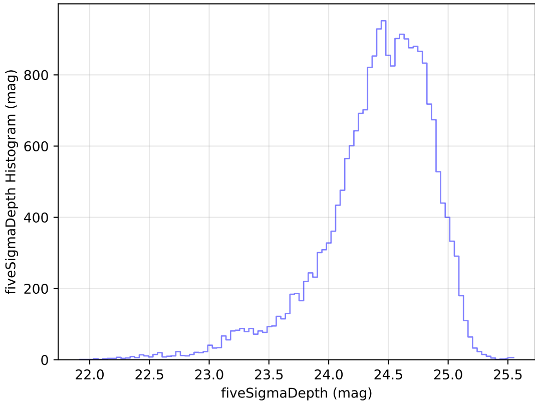
weather_cloudso1v3.4_10yrs Yr 1 g band: fiveSigmaDepth Histogram
