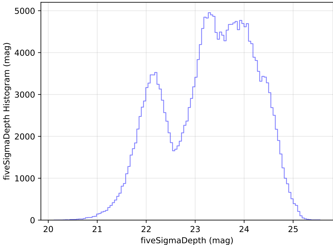
weather_cloudso1v3.4_10yrs Yr 1 all bands: fiveSigmaDepth Histogram
