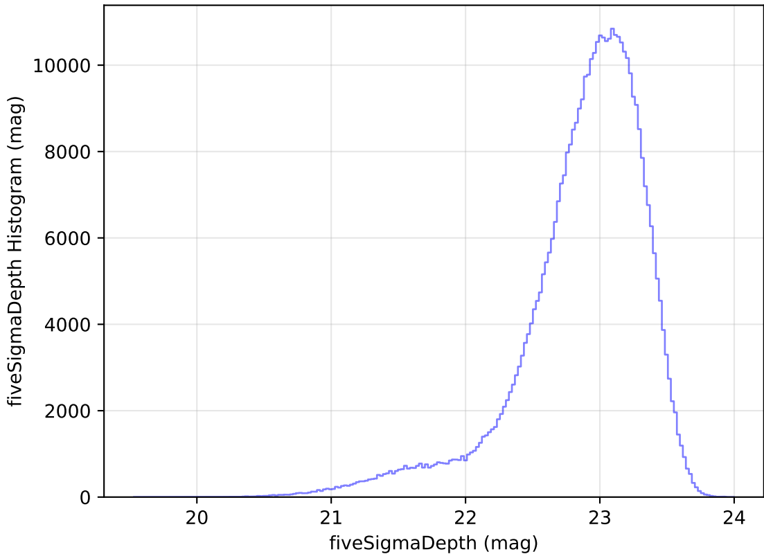
weather_cloudso1v3.4_10yrs WFD z band: fiveSigmaDepth Histogram
