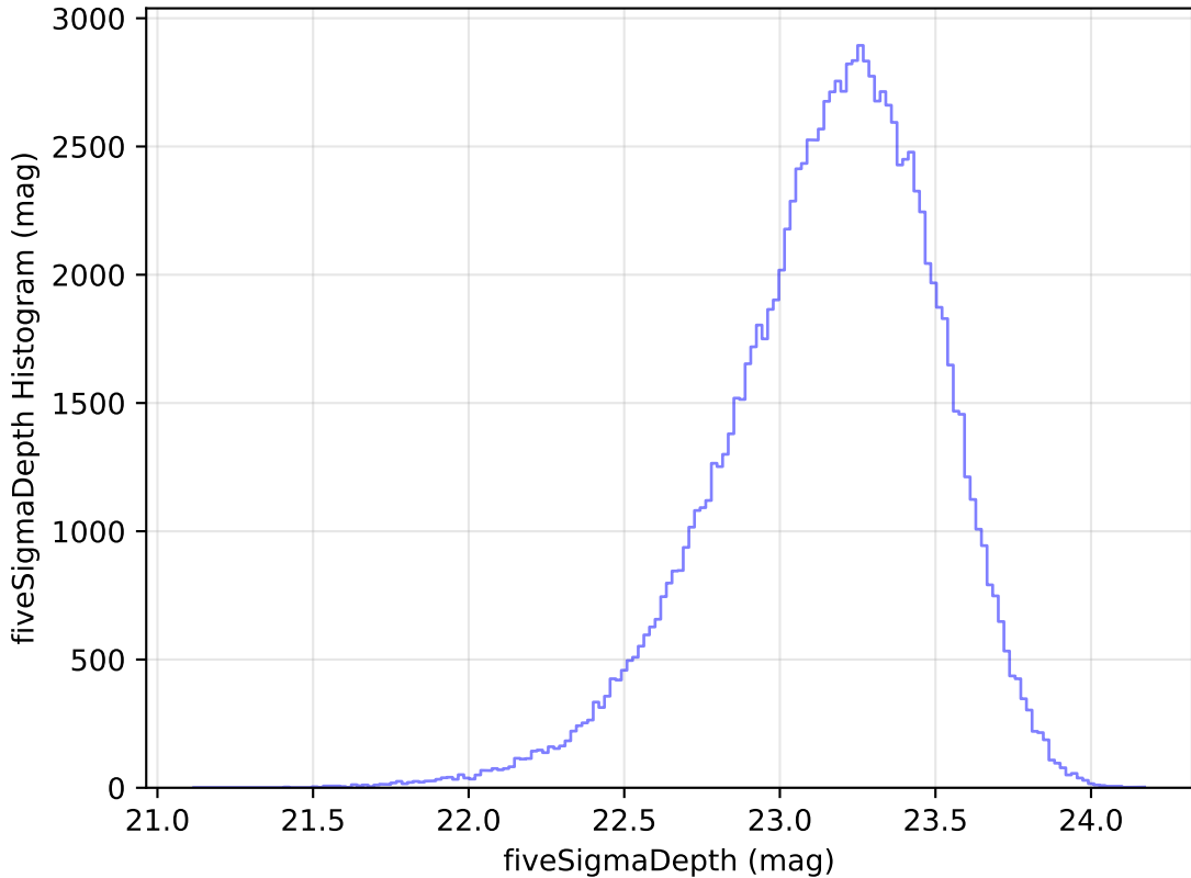
weather_cloudso1v3.4_10yrs WFD u band: fiveSigmaDepth Histogram
