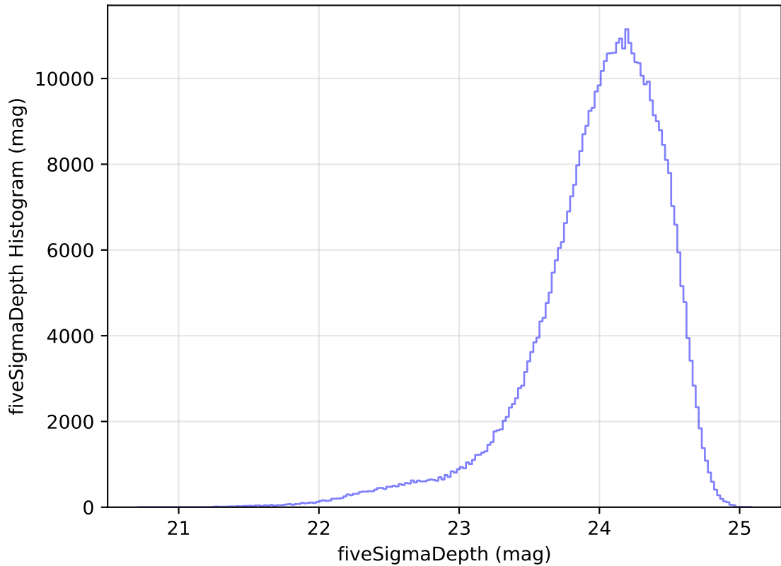
weather_cloudso1v3.4_10yrs WFD r band: fiveSigmaDepth Histogram
