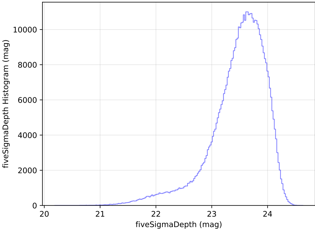
weather_cloudso1v3.4_10yrs WFD i band: fiveSigmaDepth Histogram
