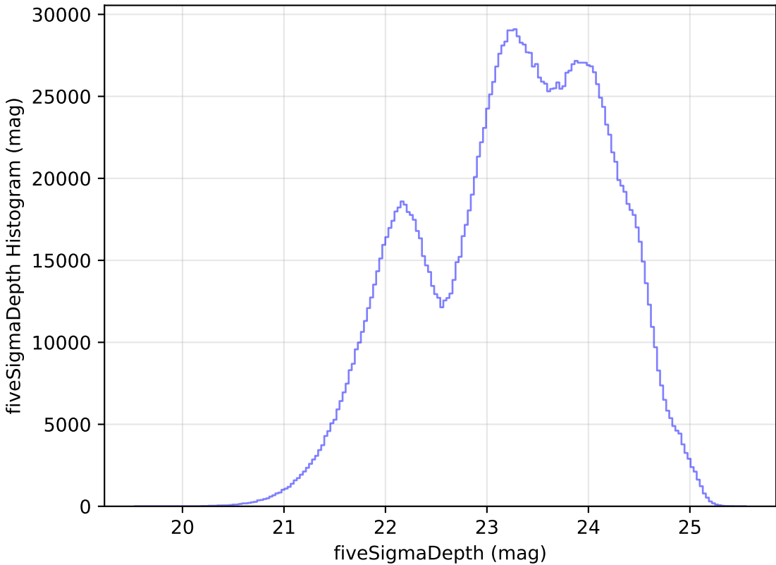
weather_cloudso1v3.4_10yrs WFD all bands: fiveSigmaDepth Histogram
