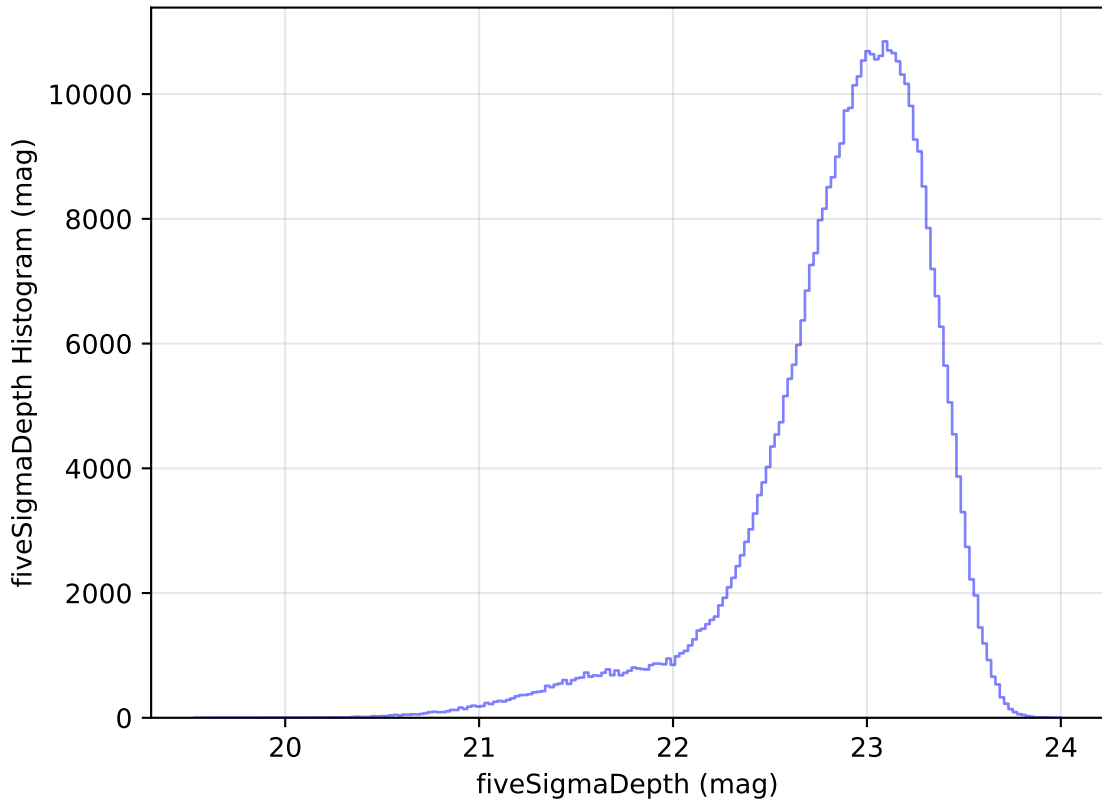
weather_cloudso1v3.4_10yrs All sky z band: fiveSigmaDepth Histogram
