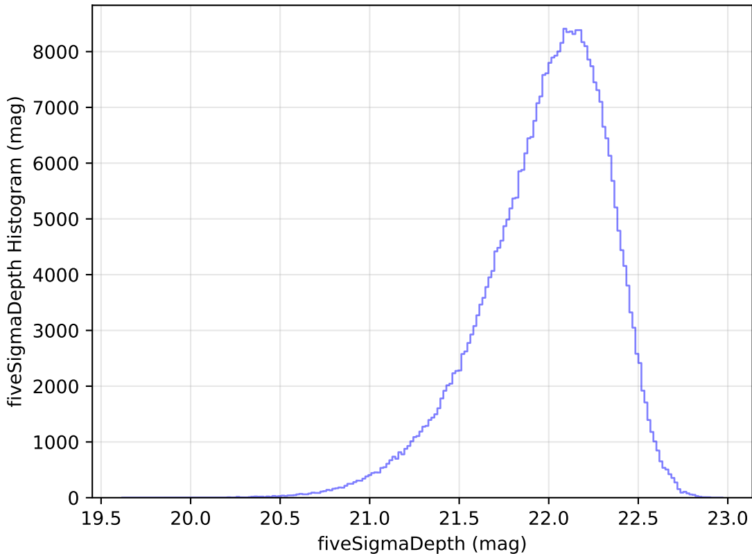
weather_cloudso1v3.4_10yrs All sky y band: fiveSigmaDepth Histogram
