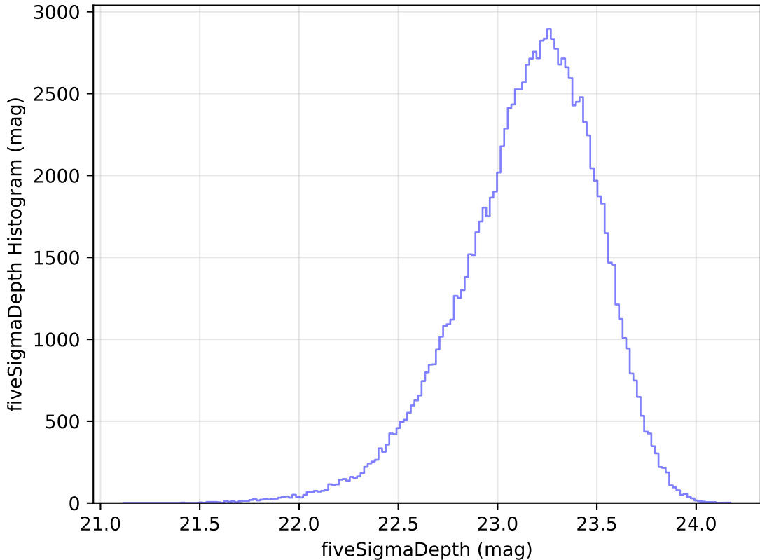
weather_cloudso1v3.4_10yrs All sky u band: fiveSigmaDepth Histogram
