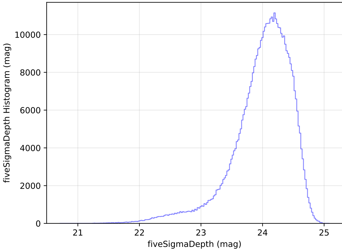
weather_cloudso1v3.4_10yrs All sky r band: fiveSigmaDepth Histogram
