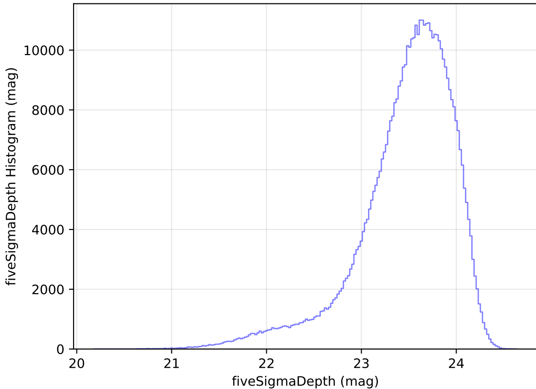
weather_cloudso1v3.4_10yrs All sky i band: fiveSigmaDepth Histogram
