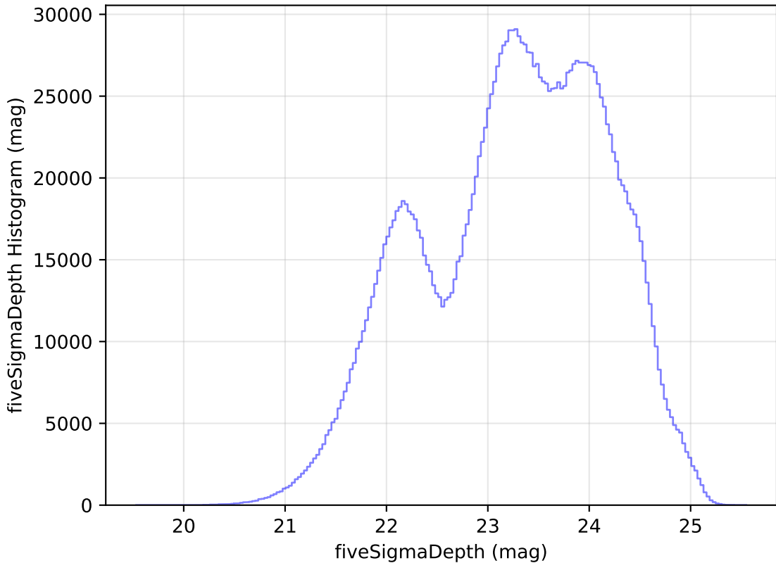
weather_cloudso1v3.4_10yrs All sky all bands: fiveSigmaDepth Histogram
