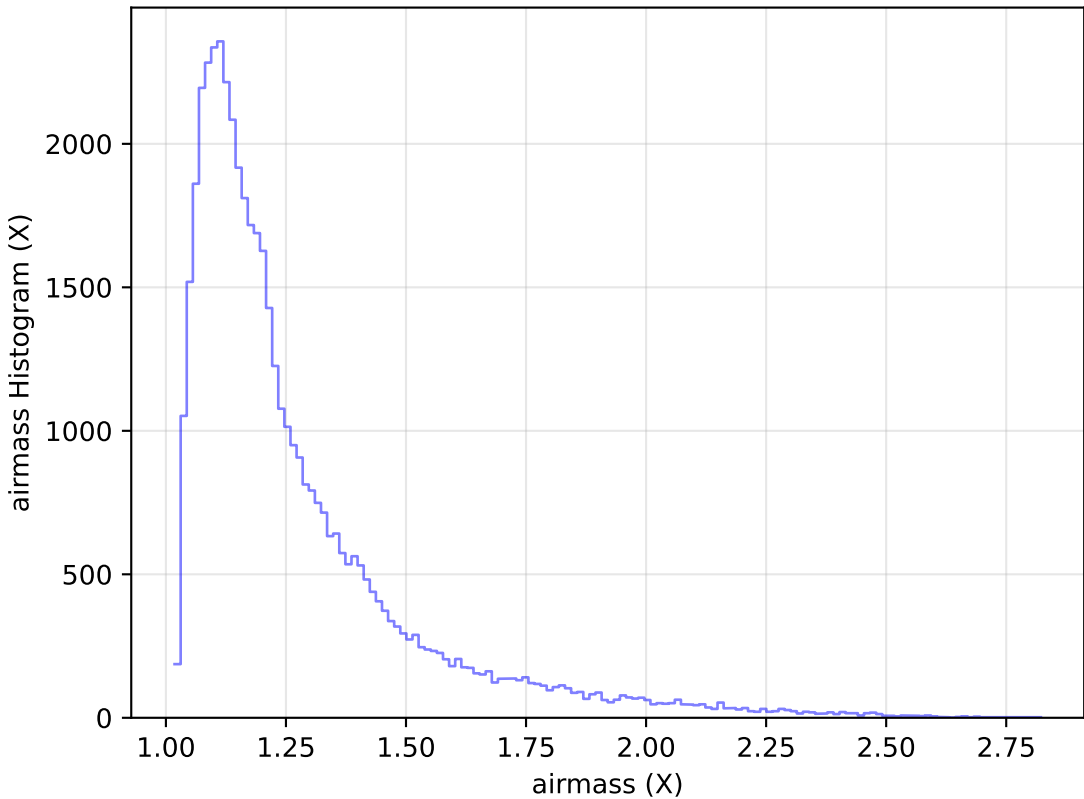
weather_cloudso1v3.4_10yrs Yr 1 y band: airmass Histogram
