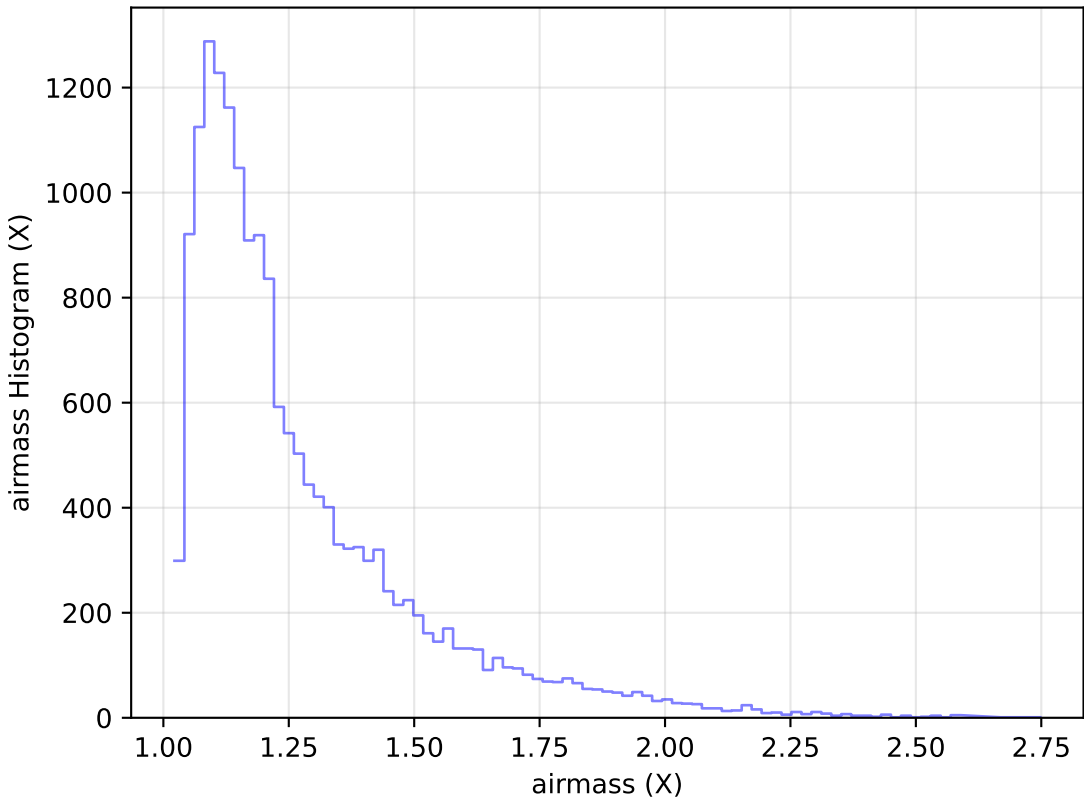
weather_cloudso1v3.4_10yrs Yr 1 u band: airmass Histogram
