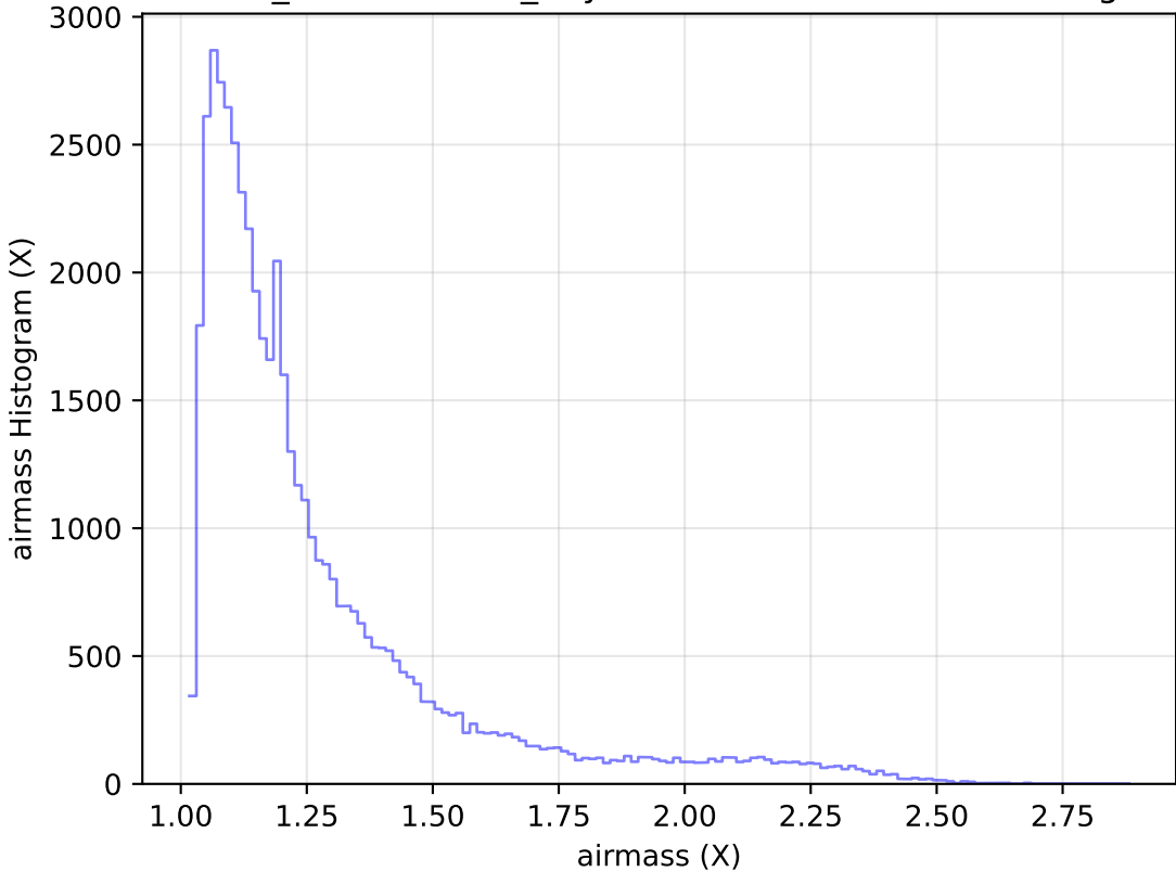
weather_cloudso1v3.4_10yrs Yr 1 r band: airmass Histogram
