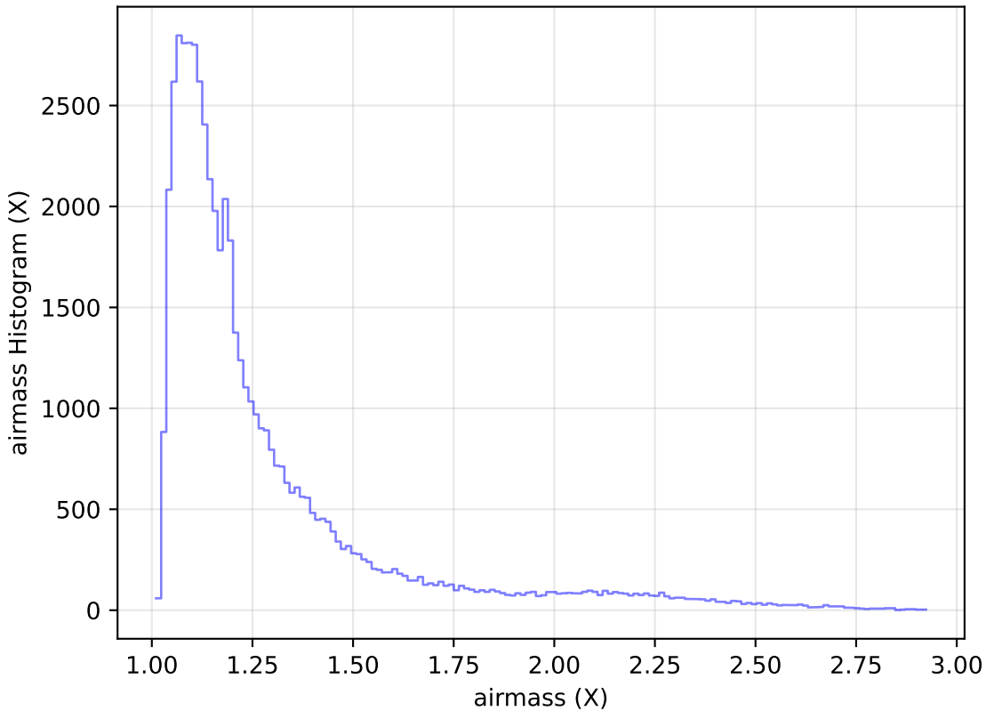
weather_cloudso1v3.4_10yrs Yr 1 i band: airmass Histogram
