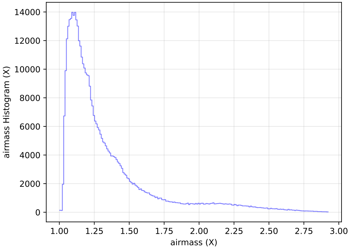
weather_cloudso1v3.4_10yrs WFD z band: airmass Histogram
