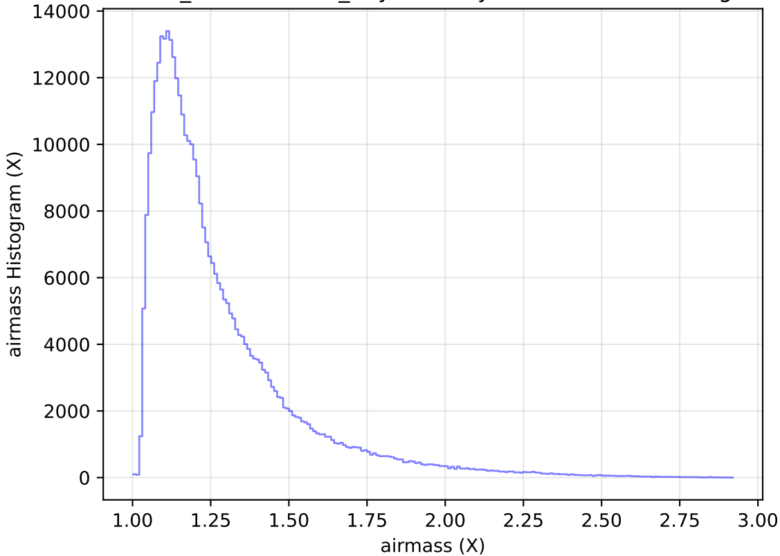
weather_cloudso1v3.4_10yrs WFD y band: airmass Histogram
