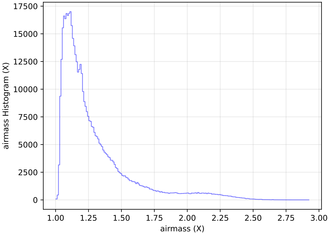
weather_cloudso1v3.4_10yrs WFD r band: airmass Histogram
