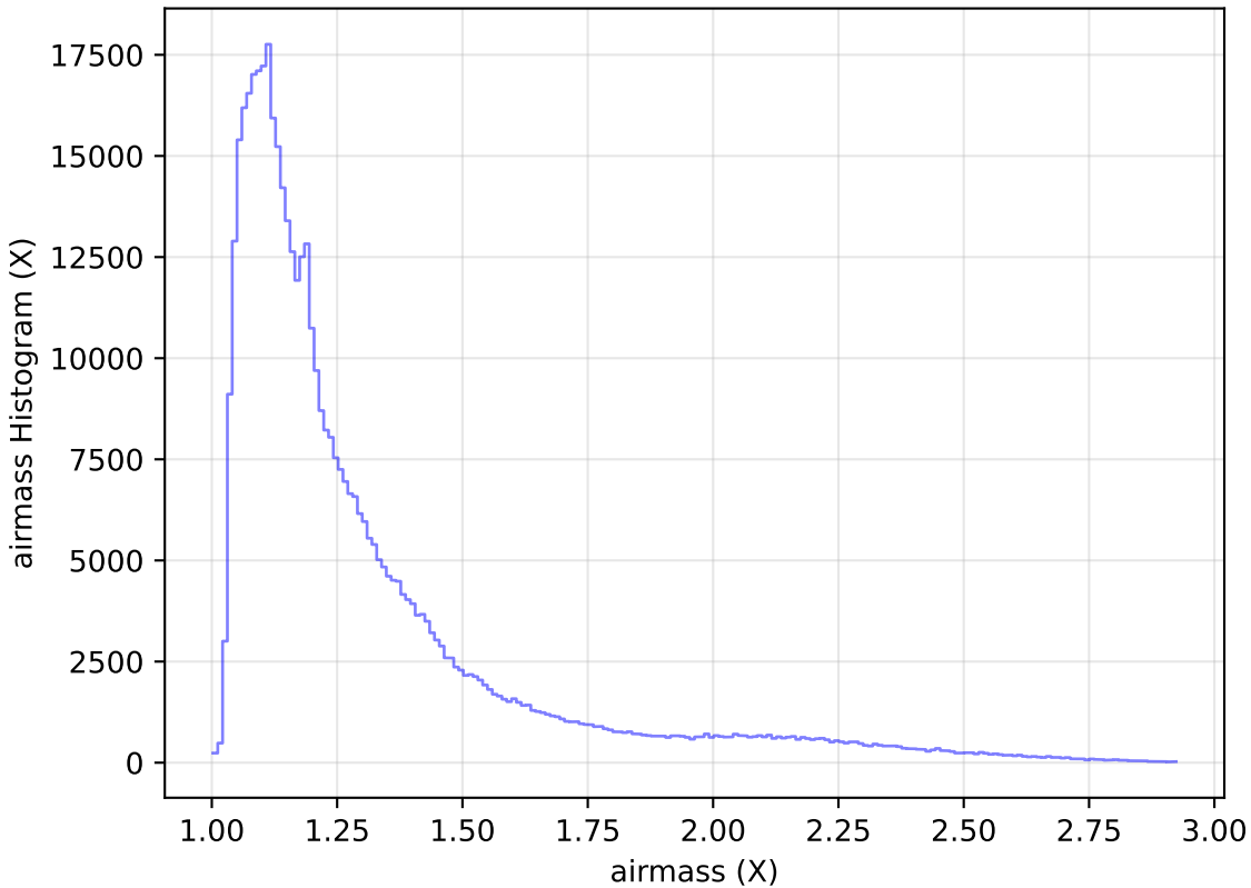
weather_cloudso1v3.4_10yrs WFD i band: airmass Histogram
