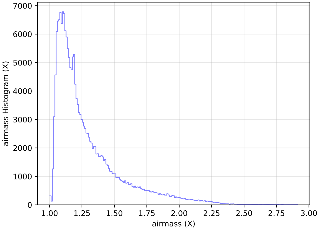
weather_cloudso1v3.4_10yrs WFD g band: airmass Histogram
