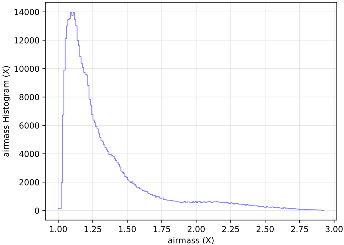
weather_cloudso1v3.4_10yrs All sky z band: airmass Histogram
