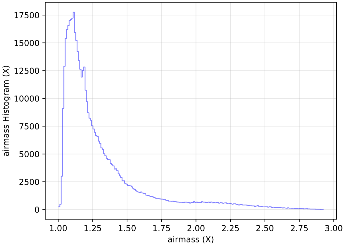
weather_cloudso1v3.4_10yrs All sky i band: airmass Histogram
