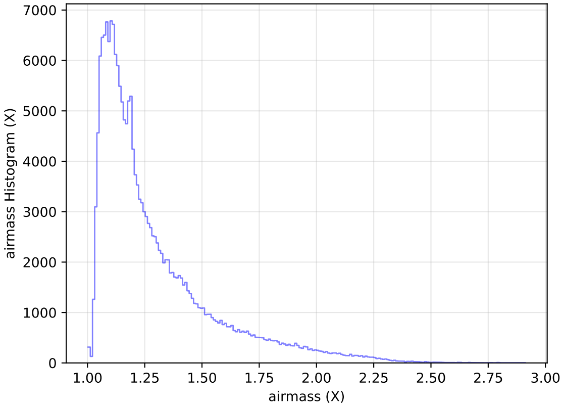
weather_cloudso1v3.4_10yrs All sky g band: airmass Histogram
